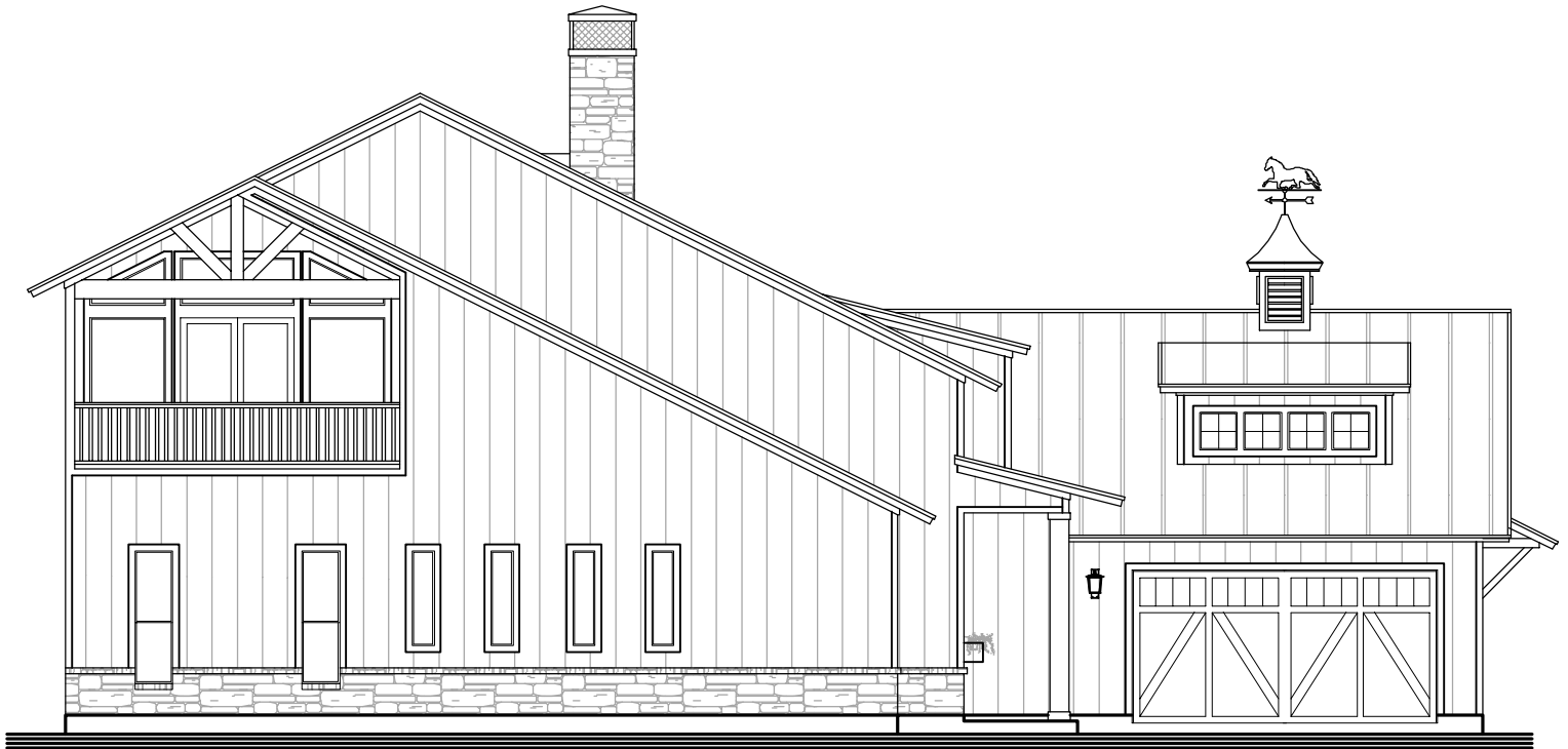
LEFT ELEVATION
